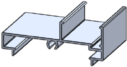
Jamba - EXA193
