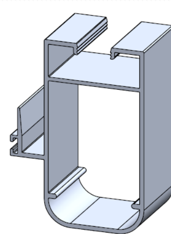
Enganche – EXA841
